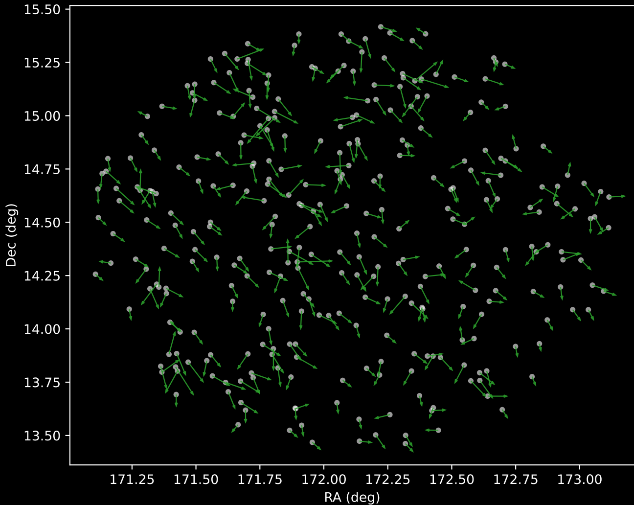
GALAH DR4 Cluster 4 Proper Motion Vectors (n=312)
