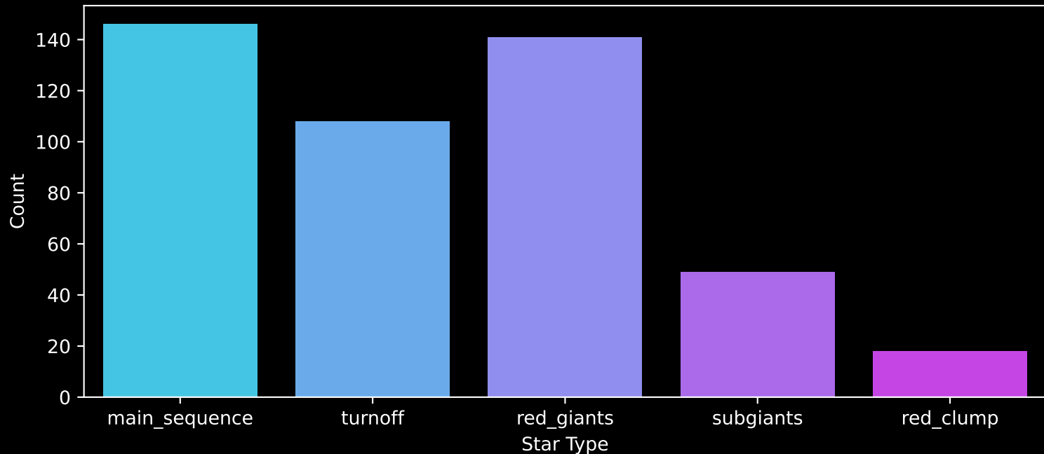
GALAH DR4 Field: [6785] Count plot of Star Type
