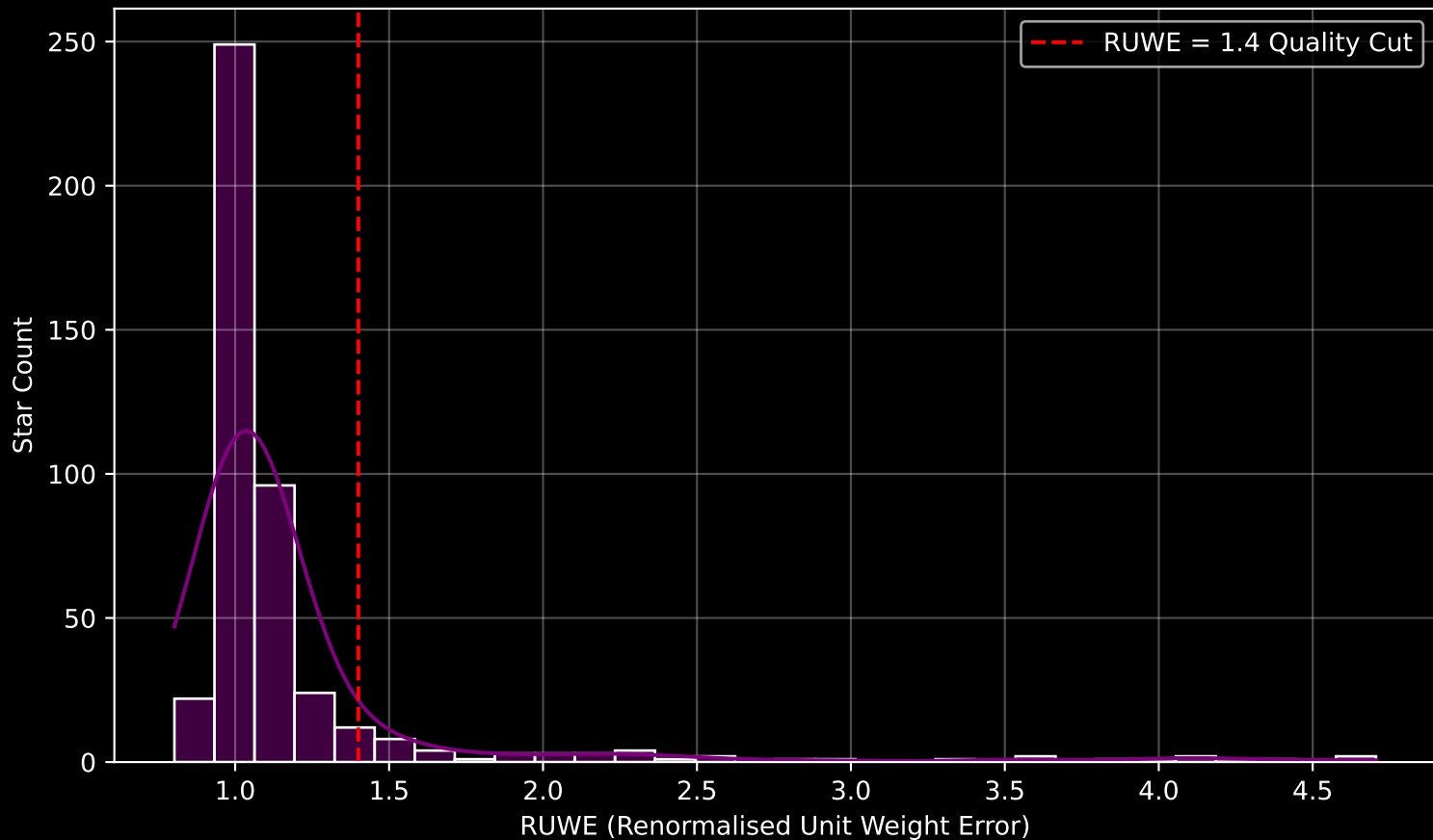
GALAH DR4 Field [6785] RUWE Distribution (n= 445)
